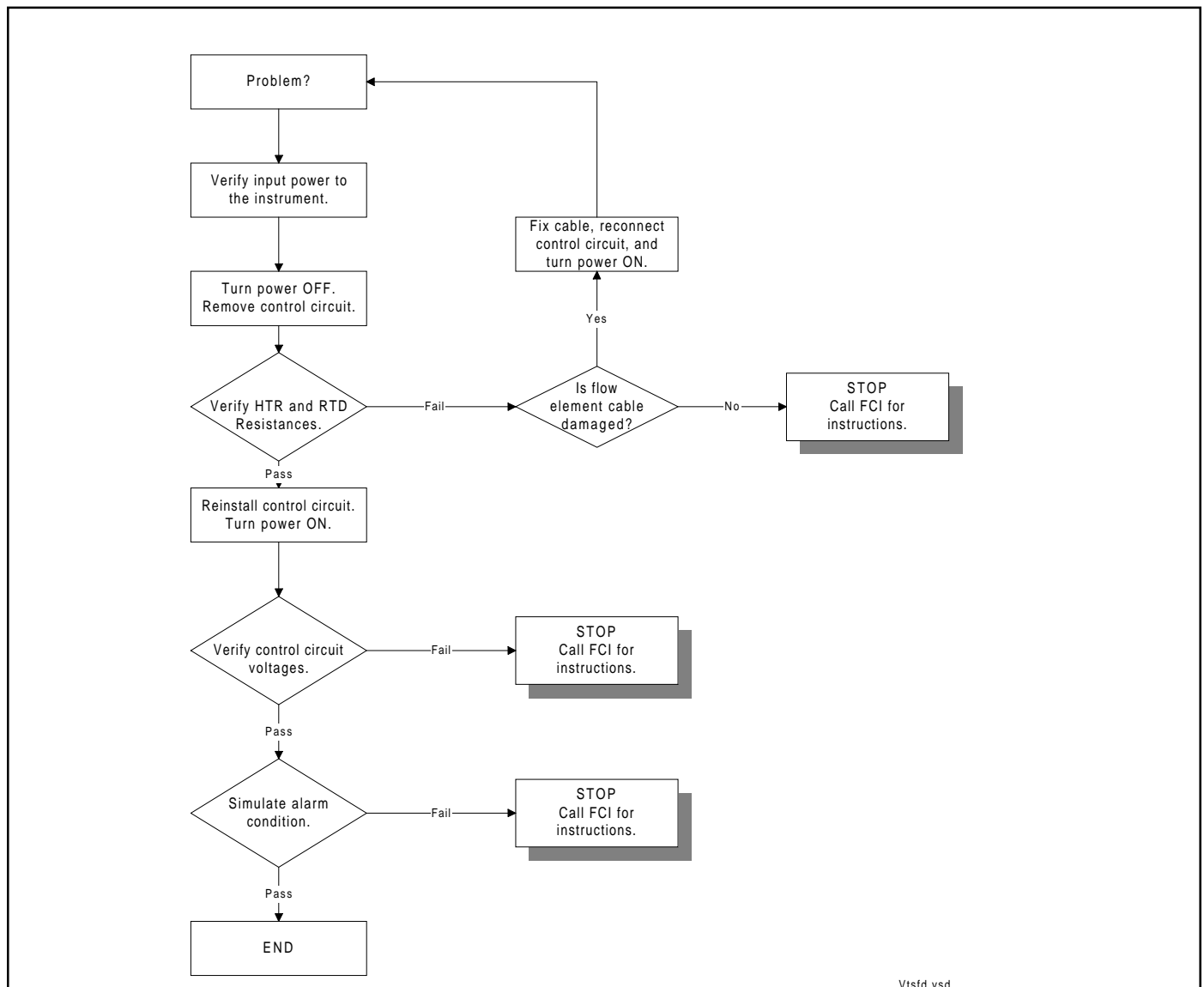
Figure 5-1. Troubleshooting Flow Chart
